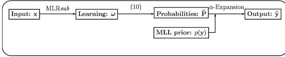
Fig. 2. Block diagram summarizing the most relevant steps of the proposed MLR_{sub}MML algorithm.
