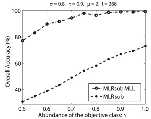
Fig. 4. OA results as a function of the abundance of the objective class: \gamma , with \tau = 0.9 , \mu = 2 , and l = 288 for a problem with mixed pixels and \sigma = 0.8 . Dash-dot lines with circles denote the segmentation results obtained by the \text{MLR}_{\text{sub}}\text{MMLL} algorithm; dashed lines with asterisks denote the classification results obtained by the \text{MLR}_{\text{sub}} algorithm.
