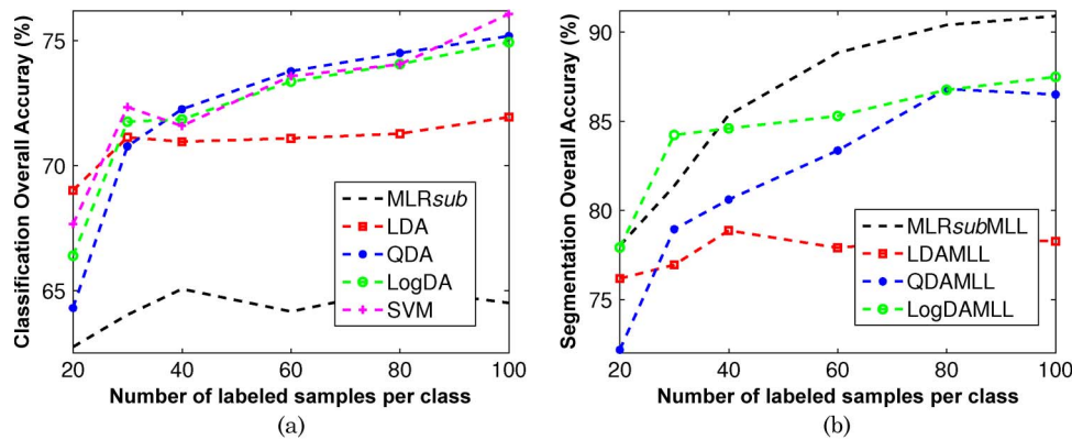
Fig. 12. OA results as a function of the number of labeled samples per class for the University of Pavia data set. (a) Classification results. (b) Segmentation results.
