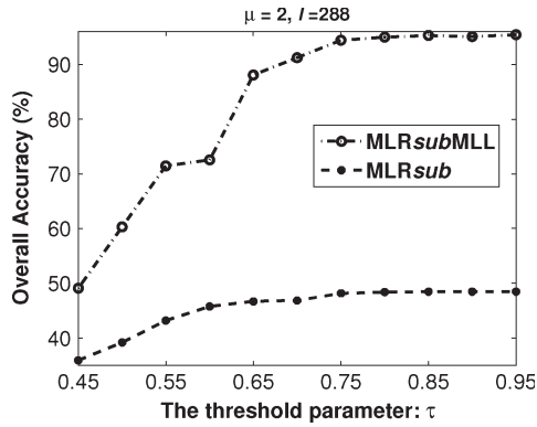
Fig. 5. OA results (as a function of \tau ) with \mu = 2 for a problem with \sigma = 0.8 and \gamma = 0.7 .
