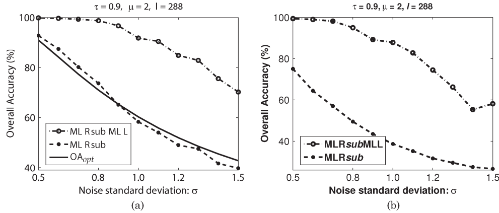
Fig. 8. OA results achieved (for two different values of \gamma ) as a function of the noise standard deviation \sigma with \tau = 0.9 , \mu = 2 , and l = 288 . (a) \gamma = 1 . (b) \gamma = 0.7 .
