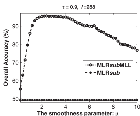
Fig. 7. OA results as a function of the smoothness parameter \mu for a problem with \sigma = 0.8 and \gamma = 0.7 with \tau = 0.9 and l = 288 .
