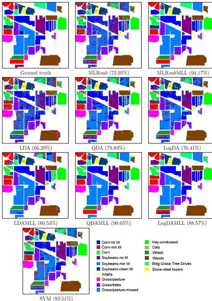
Fig. 9. Classification/segmentation maps obtained by the different tested methods for the AVIRIS Indian Pines scene (overall accuracies are reported in parentheses).
