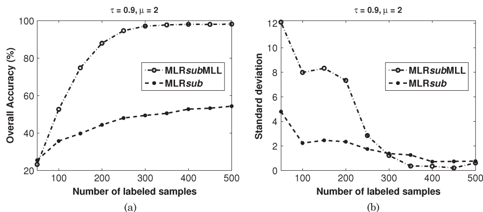
Fig. 6. Classification and segmentation results obtained for a problem with \sigma = 0.8 and \gamma = 0.7 by using \tau = 0.9 and \mu = 2 . (a) OA results as a function of the number of labeled samples. (b) Standard deviation results as a function of the number of labeled samples.
