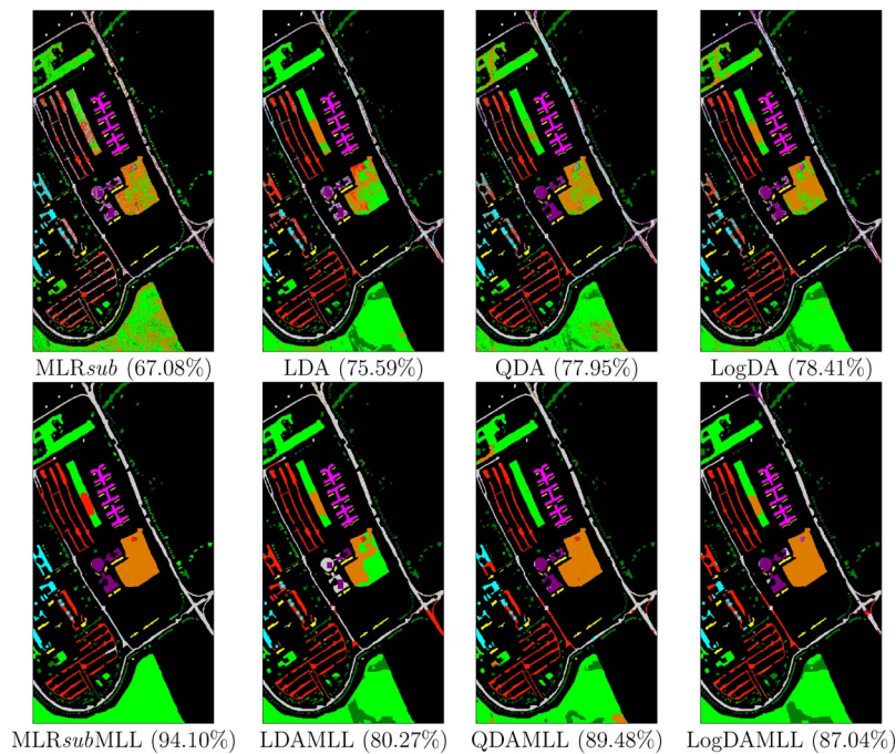
Fig. 11. Classification/segmentation maps obtained by the different tested methods for the ROSIS University of Pavia scene (overall accuracies are reported in parentheses).
