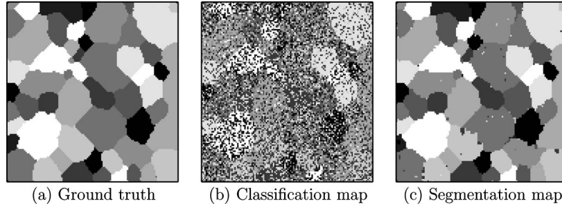
Fig. 3. Classification and segmentation maps obtained after applying the proposed method to a simulated hyperspectral scene with \sigma = 0.8 and \gamma = 0.7 by using \tau = 0.9 , l = 288 , and \mu = 2 . (a) Ground-truth class labels. (b) Classification result (OA = 49.09%). (c) Segmentation result (OA = 94.34%).
