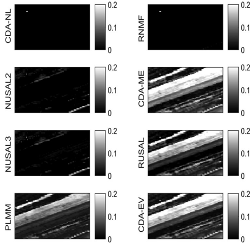
Fig. 11. Residual maps for the Salinas image obtained with \|\hat{y}_{i,j} - M\hat{a}_{i,j}\| .
