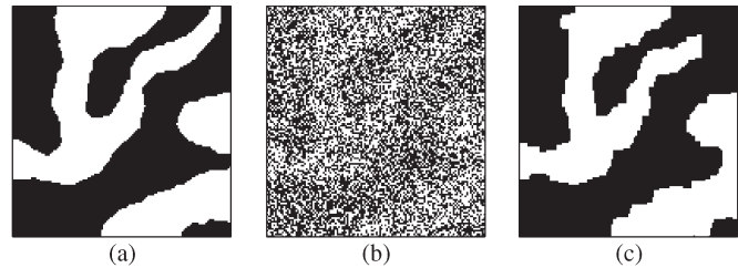
Fig. 4. Classification and segmentation results obtained with the proposed algorithm. The simulated data set was generated according to (18) with d = 500 , \sigma = 1.5 , and \mu = 2 . (a) Simulated binary map. (b) Classification map produced by the LORSAL algorithm using L = 100 labeled samples without active learning (OA = 60.13%, with OA_{opt} = 71.91\% , see text). (c) Segmentation map, same as (b) but using the MLL spatial prior (OA = 92.48%).
